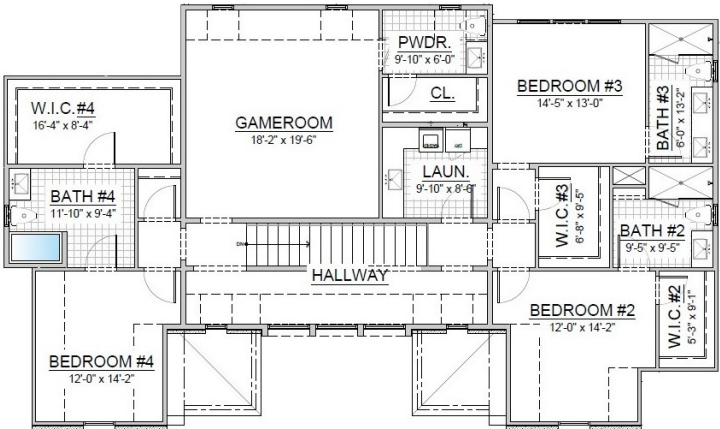
2nd Floor
