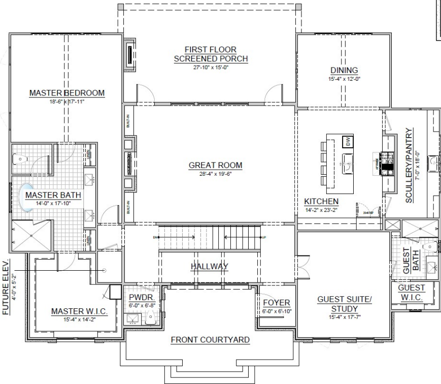
1st Floor
